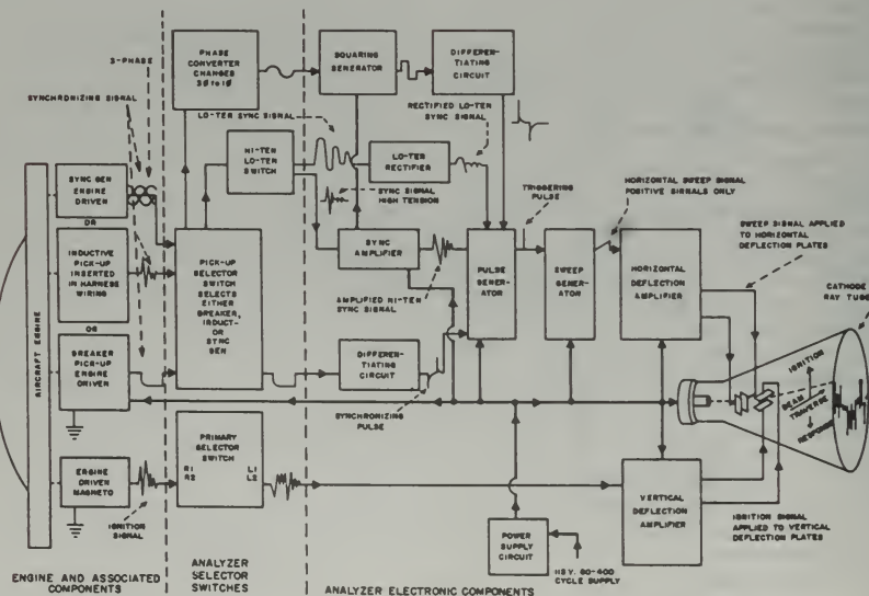
FIGURE 4-73. Diagram of ignition analyzer.
